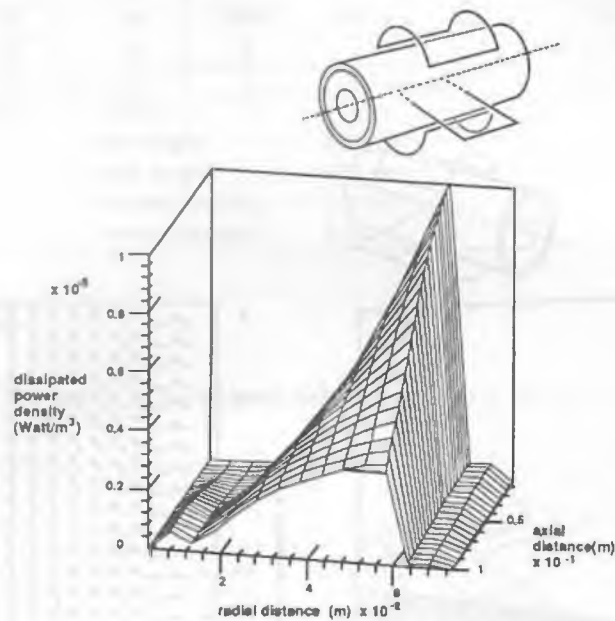
Fig.4 Local density of dissipated power.
